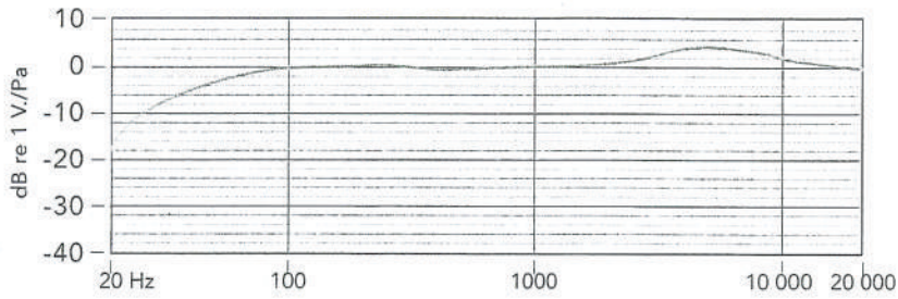
FREQUENCY RESPONSE
